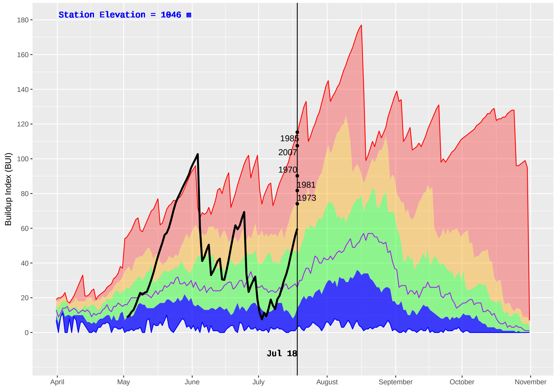
LIKELY RS (255) : Historical (1970–2016) and Current (2018) Daily Buildup Index (BUI)
