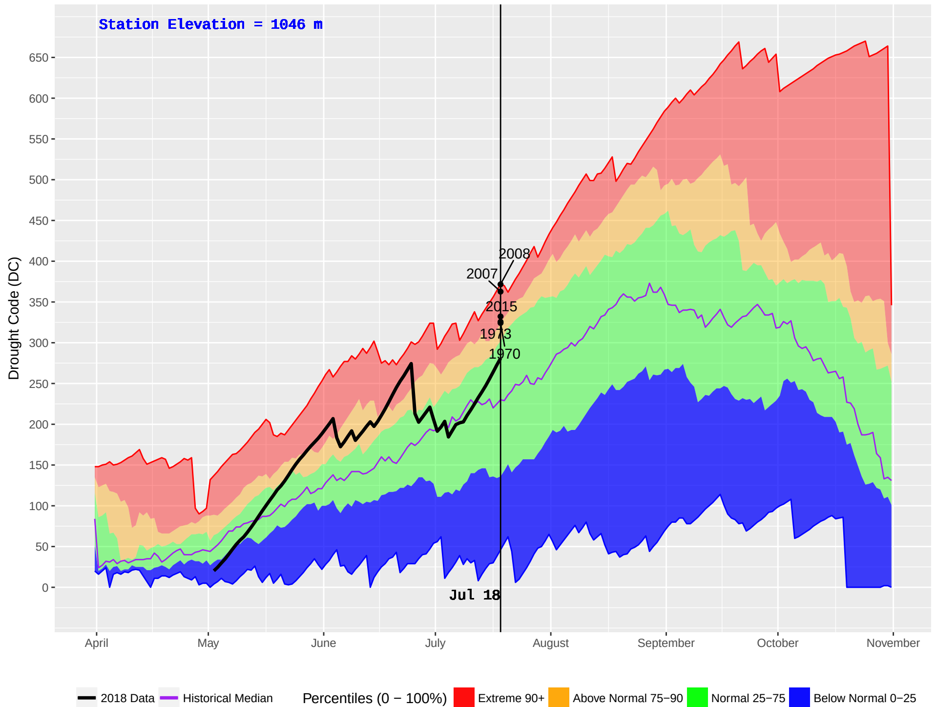
LIKELY RS (255) : Historical (1970–2016) and Current (2018) Daily Drought Code (DC)
