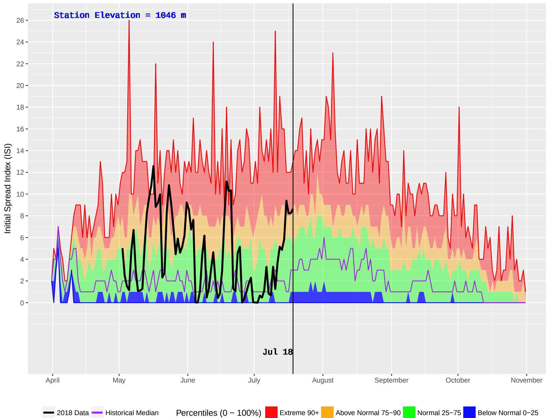
LIKELY RS (255) : Historical (1970–2016) and Current (2018) Daily Initial Spread Index (ISI)
