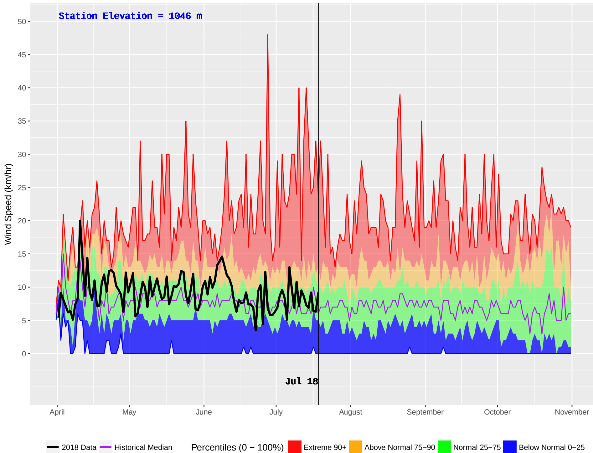
LIKELY RS (255) : Historical (1970–2016) and Current (2018) Daily Wind Speed
