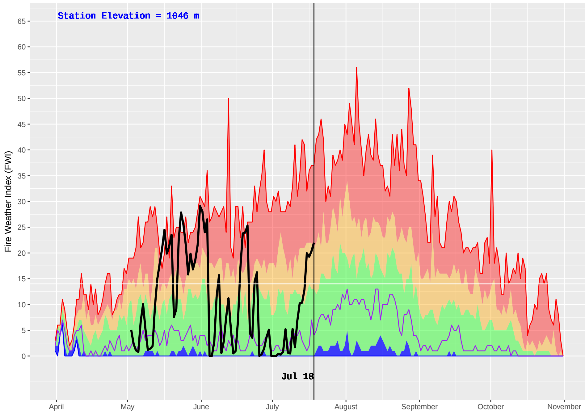
LIKELY RS (255) : Historical (1970–2016) and Current (2018) Daily Fire Weather Index (FWI)
