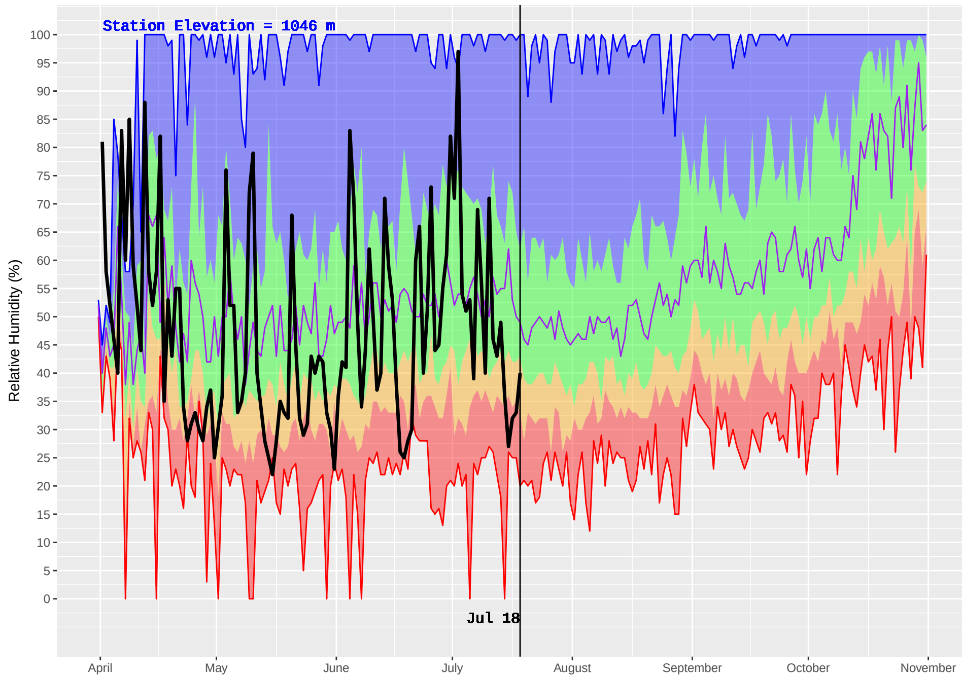
LIKELY RS (255) : Historical (1970–2016) and Current (2018) Daily Relative Humidity
