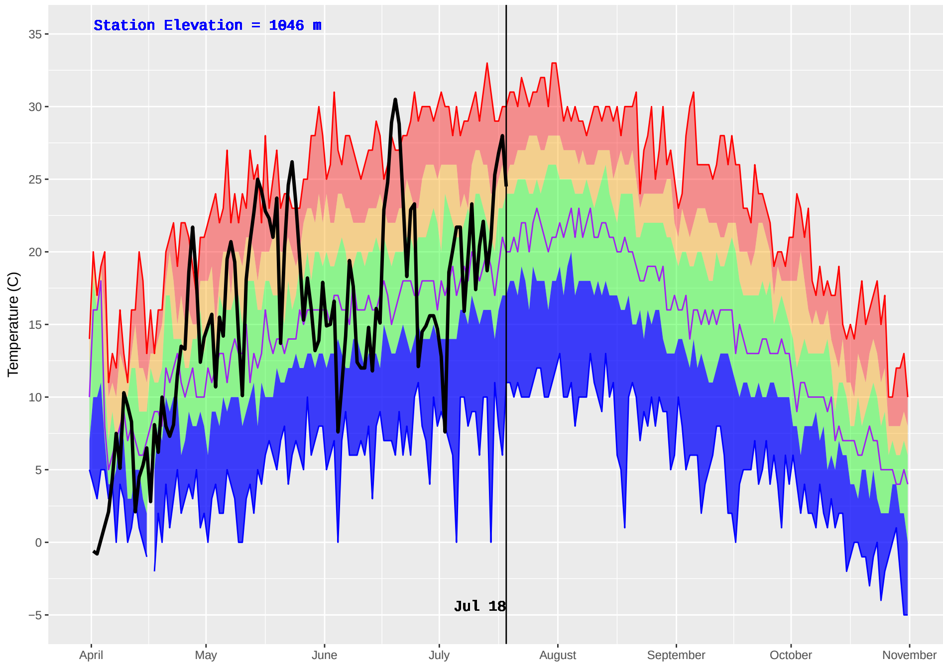
LIKELY RS (255) : Historical (1970–2016) and Current (2018) Daily Temperature
